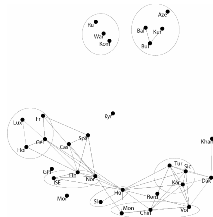
Figure 5. MDS plot of the connections of 31 folk music cultures. Connecting lines indicate the mutually largest relative overlaps.
